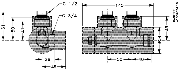
VHS angle pattern 1/2 or 3/4" radiator connection
