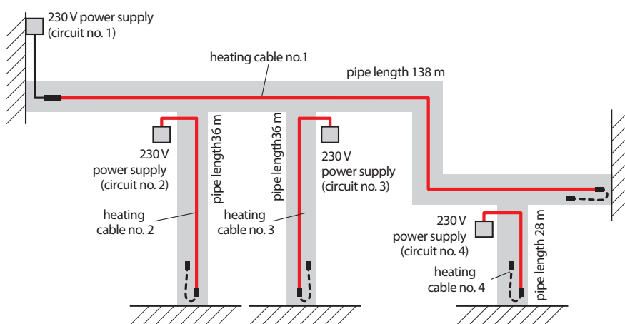
Division in circuits – constant wattage heating cables
